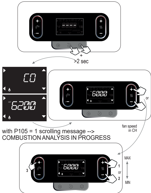
The probe for the fumes analysis must be inserted until it reaches the stop
