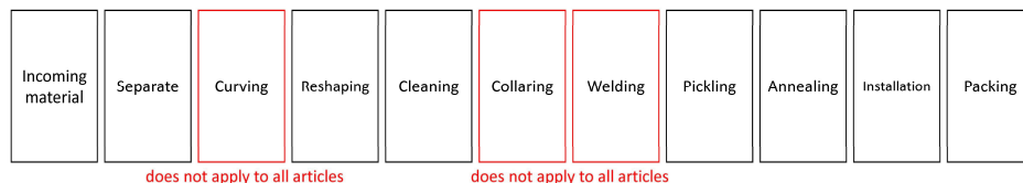
Illustration 1 Manufacturing process
