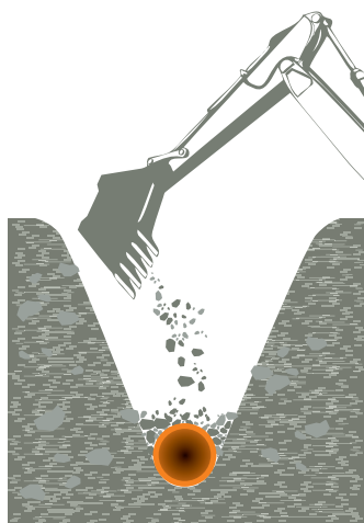
Rura PE100 RC bez podsypki
